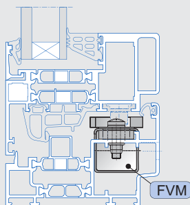
铝制窗
