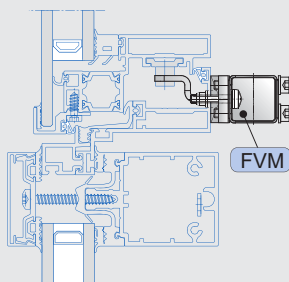
铝制窗
