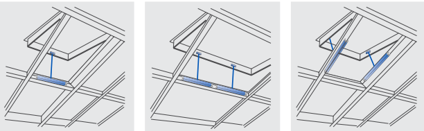
采光顶
